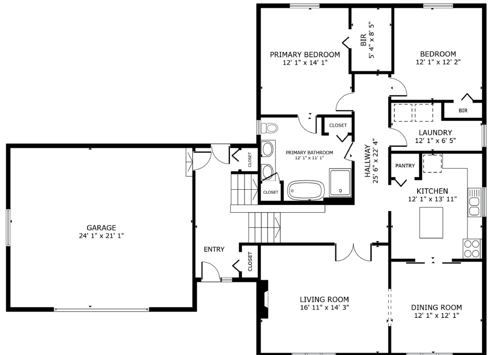
FLOOR 2
