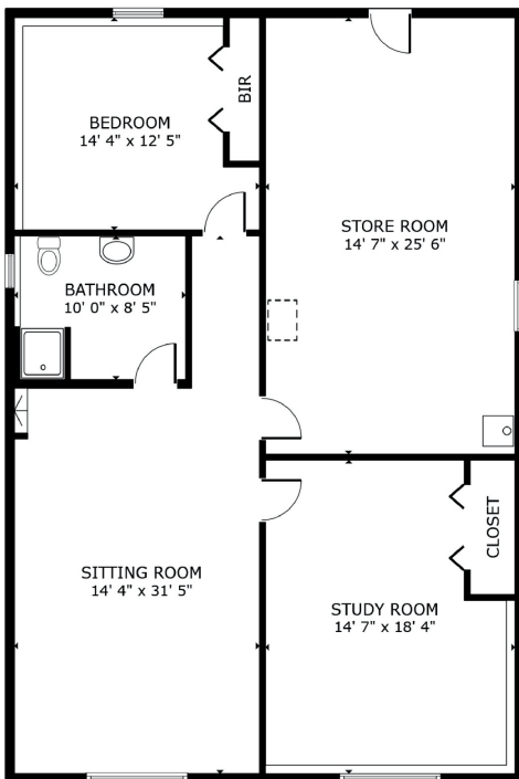
FLOOR 1
