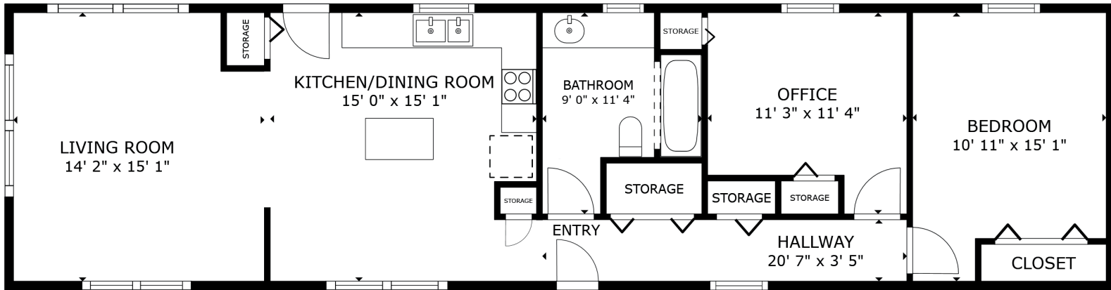
FLOOR PLAN
