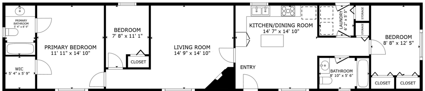
FLOOR PLAN
