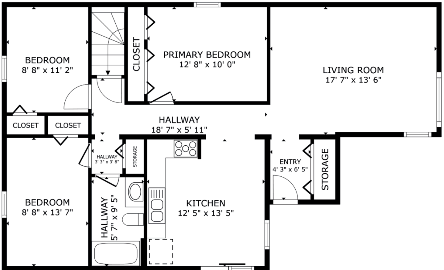
FLOOR 2
